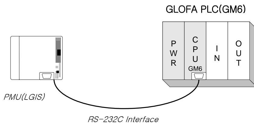
The example of 1:1 connection with LGIS protocol (Cnet connection with PMU)
